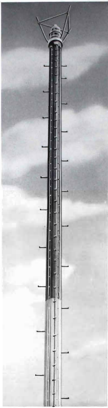
FIG. 4. The RCA TFU-30J UHF-Pylon Antenna. Offering a power gain of 30, this pylon is capable of 1.5 megawatts of ERP with a power input of 50 kw.
