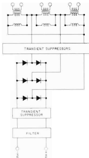
FIG. 5. Modified rectifier circuit using silicon rectifiers (simplified schematic).
