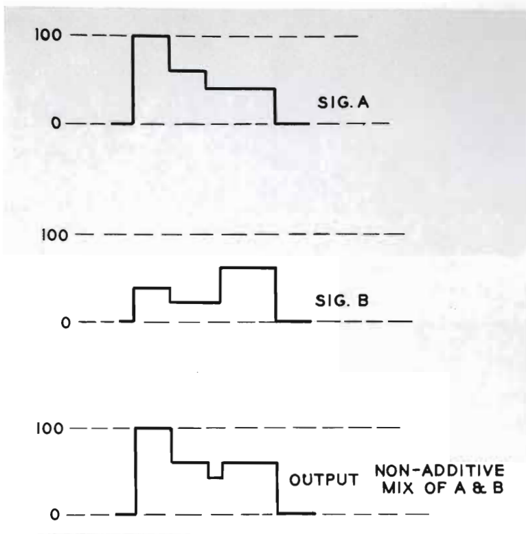
FIG. 13. Non-additive mixing of two signals, A and B, produces an output signal having only the highest amplitudes of either A or B.
