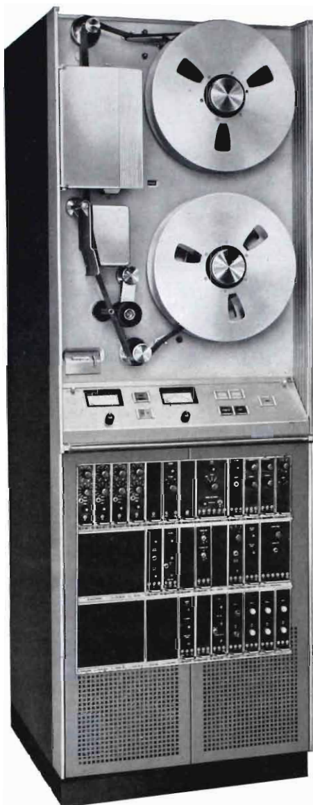
FIG. 6. TR-3 TV Tape Player, with bottom doors removed to reveal the modular construction.
