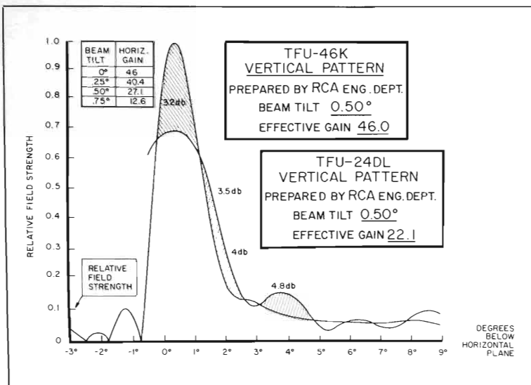
FIG. 1. Comparison of the field-strength curves between a 46- and a 24-gain antenna under identical circumstances. The shaded area shows the regions of increase or decrease in field strength when one antenna is substituted directly for the other.
