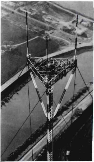
FIG. 6. This "California Candelabra" is typical of the candelabra-tower antennas now operating in Maryland, Texas and California. UHF antennas require far less spacing than do VHF.
