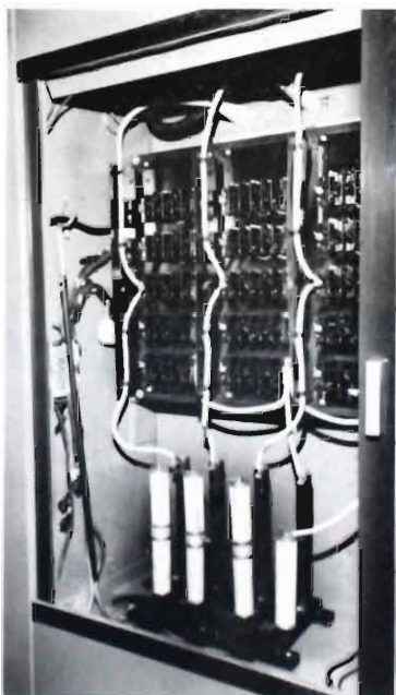
FIG. 7. Front view TTU-25B rectifier cabinet at WBRE-TV, showing new silicon rectifier stacks.
