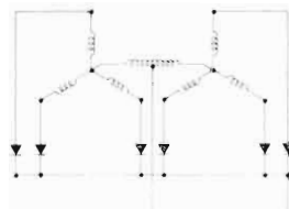
FIG. 6. Original WBRE-TV rectifier circuit using tubes (simplified schematic).
