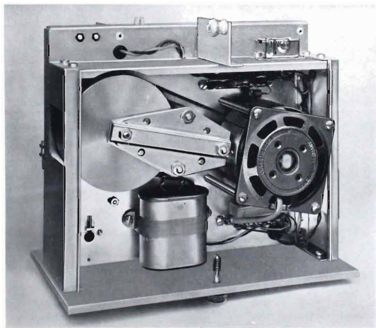
FIG. 3. The drive system for the transport includes a heavy-duty hysteresis synchronous motor and a precision ground capstan and flywheel assembly.
