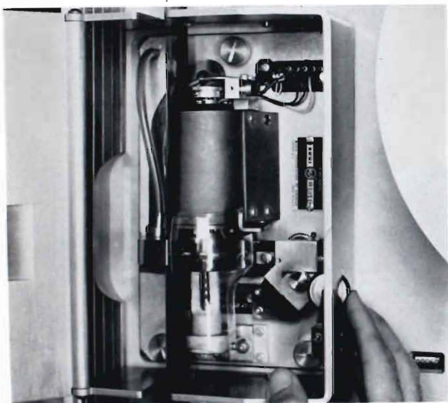
FIG. 10. Skewing adjustment of TR-3.
