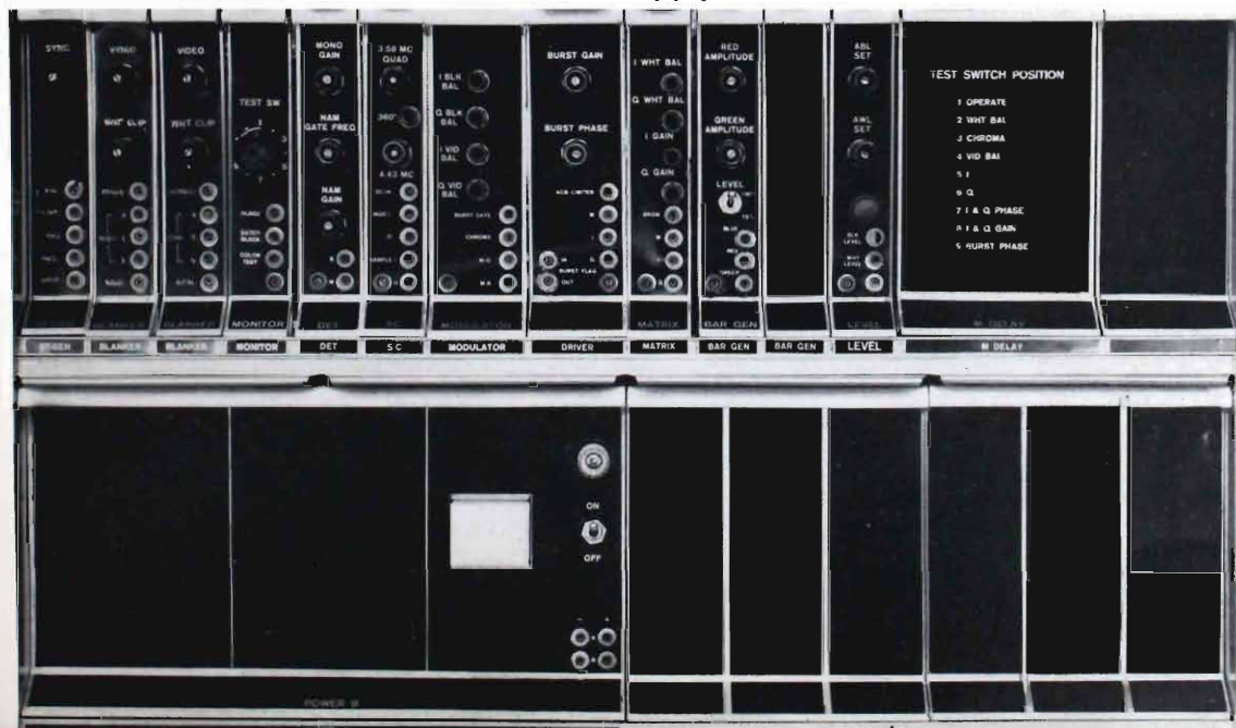
FIG. 6. Camera Auxiliary plug-in modules.
