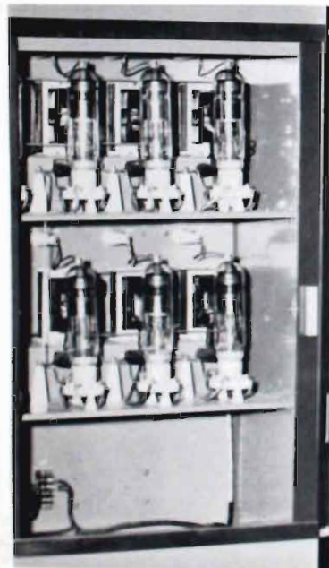
FIG. 4. Front view TTU-25B rectifier cabinet showing original tube rectifier.
