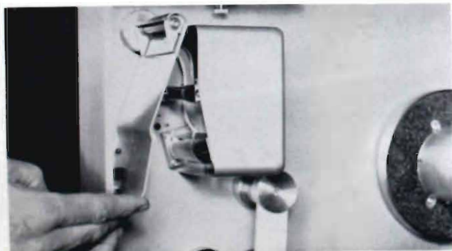
FIG. 11. Audio head of TR-3.
