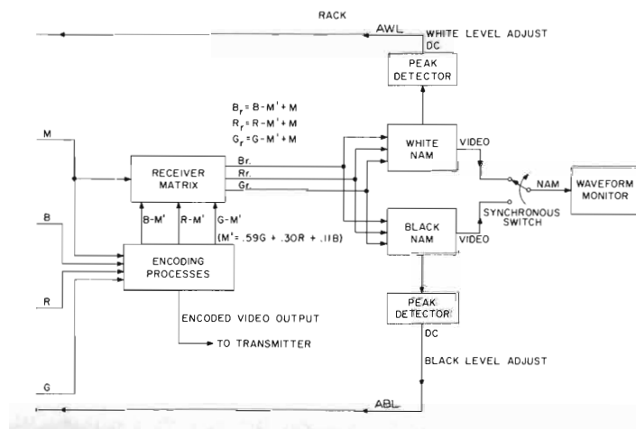
FIG. 12. Simplified block diagram of TK-27 monitoring and automatic systems.
